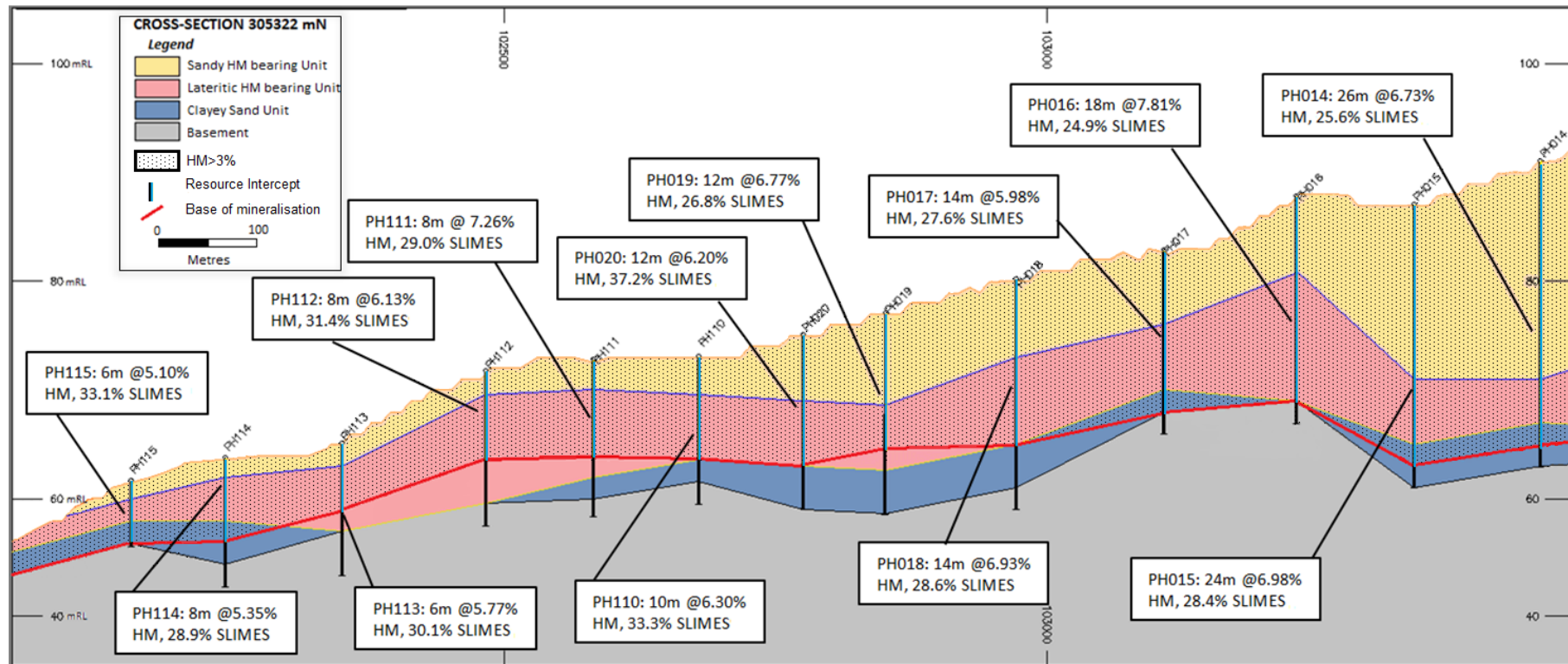
Figure 6 – EL/233 Coco resource section 305322 mN showing drill holes, intersections and principal stratigraphic units
