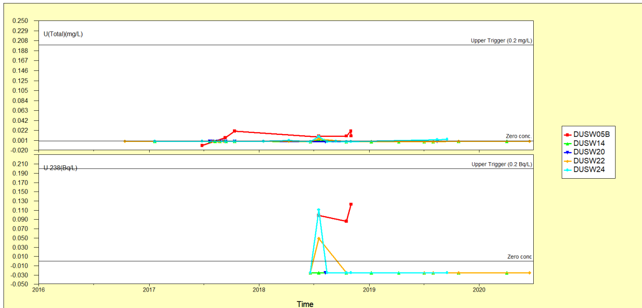
Figure 25: Uranium and U-238 in surface water
